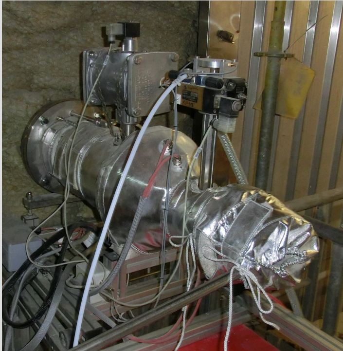
(top) filter probe with heating modules up to 200 °C - (below) filter sample is placed between the filter bags through flange
